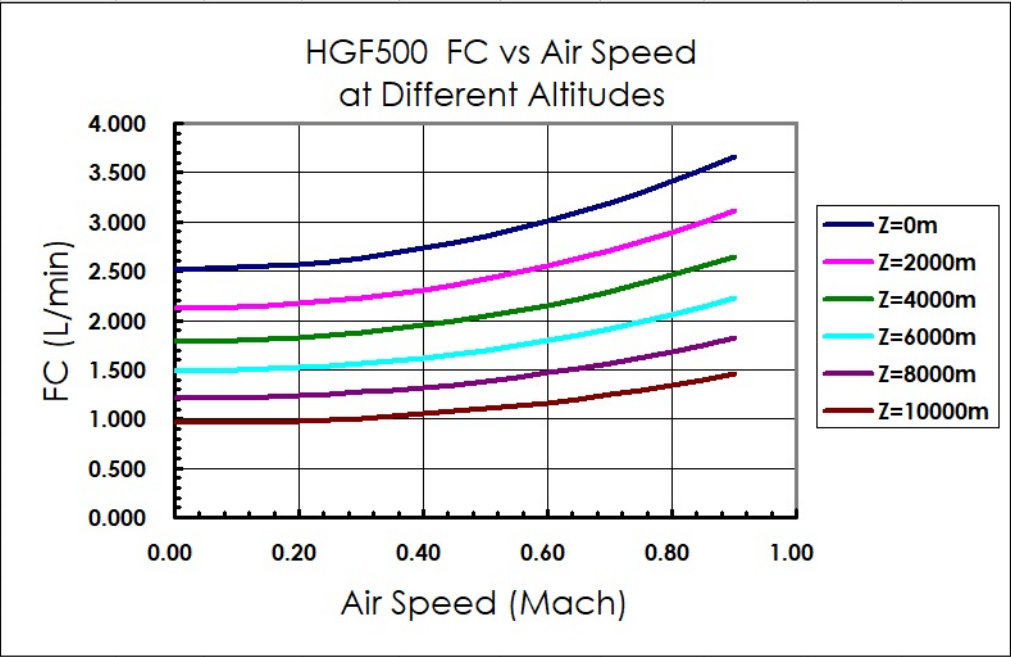
Fig 2b HGF500 Fuel Consumption at Max Thrust
