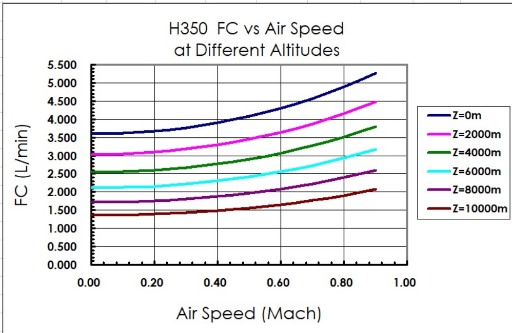
Fig 1b H350 Fuel Consumption at Max Thrust
