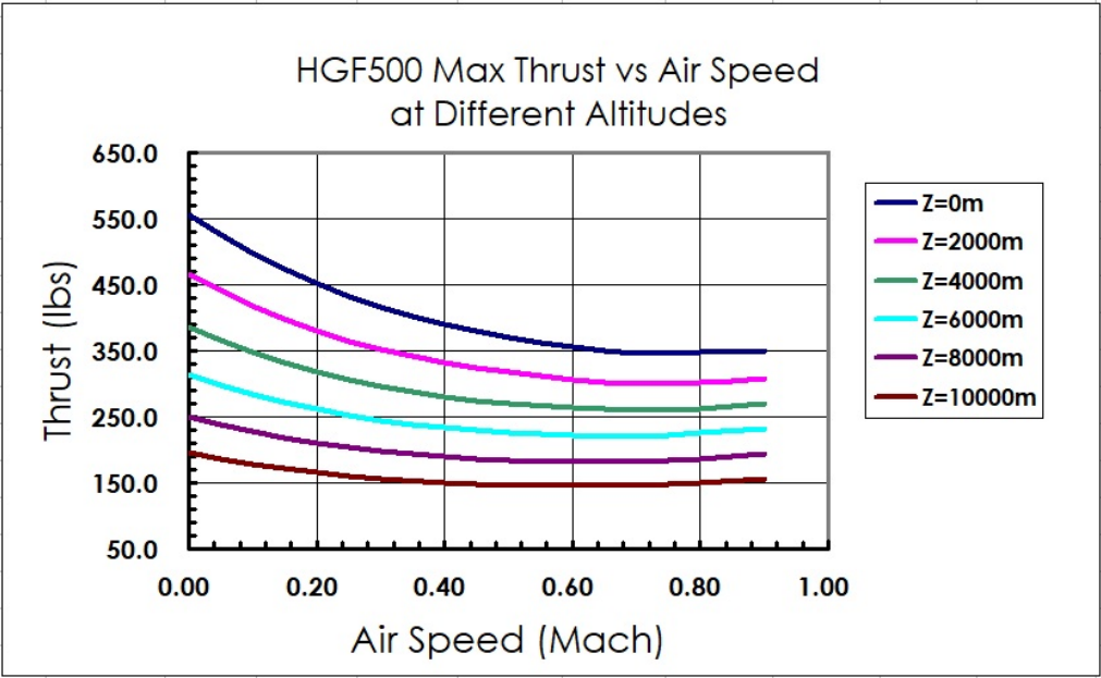
Fig 2a HGF500 Max Thrust
