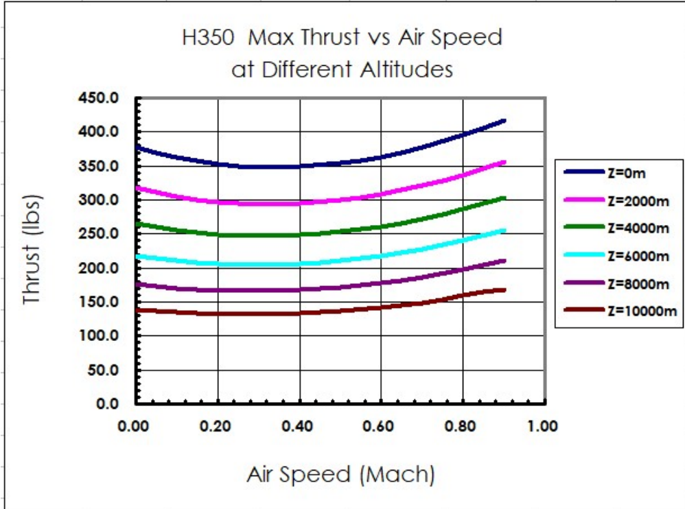
Fig 1a H350 Max Thrust
